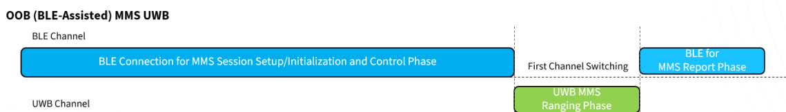
Figure 23: OOB (BLE-Assisted) MMS UWB
